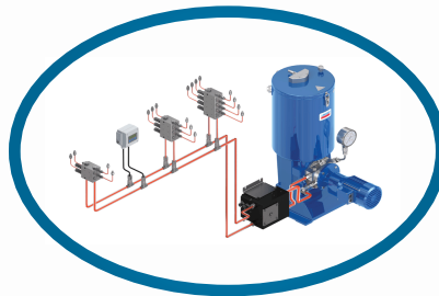
Dual-line Lubrication Systems
