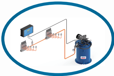
Single-line Lubrication Systems
