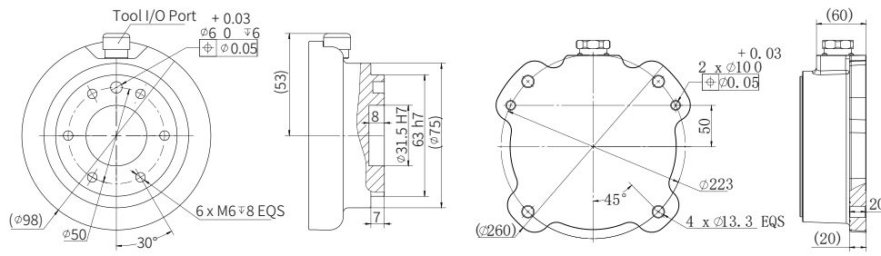
AUBO-i20 Tool End Flange
