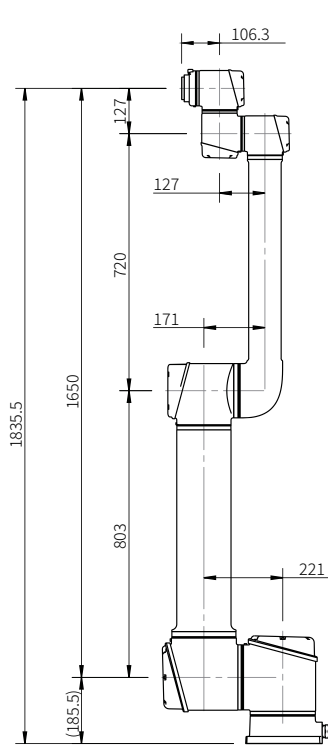
AUBO-i20 Dimensions
