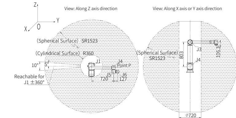
AUBO-i20 Moving Range of Point P
